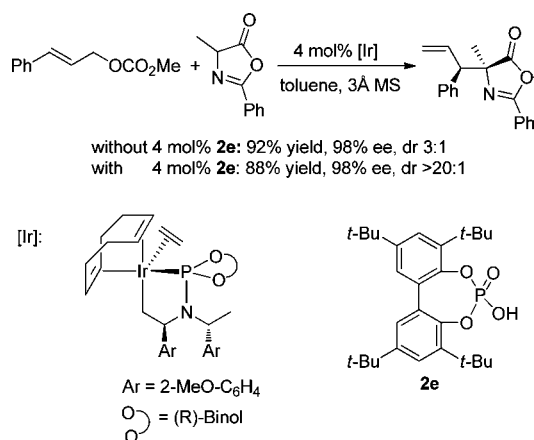
Scheme 2. Allylation of 3 Catalyzed by the Preformed Metallacyclic Iridium Catalyst with and without Phosphoric Acid 2e
