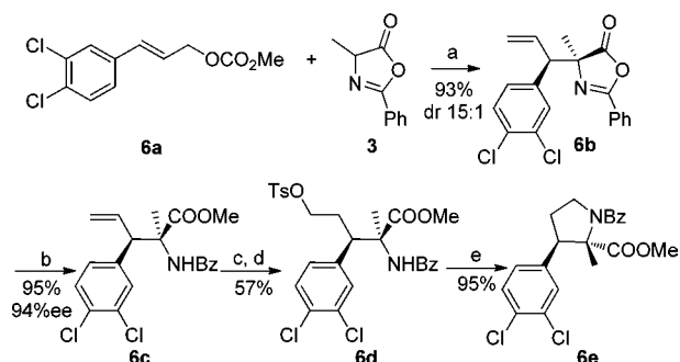
Scheme 3. Synthesis of Pyrrolidine 6e a,b
